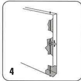
4 3-PT. LOCKING MECHANISM (on the 1A cabinet) assures total contact and sealing of door.
